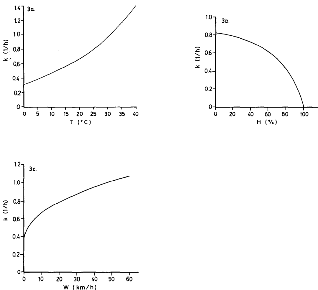
Figure 3. Variation of log drying rate k with T , H , and W in the FPMC: a) k vs T at constant H and W , b) k vs H at constant T and W , c) k vs W at constant T and H . Constant values are T = 21.1^\circ\text{C} , H = 45\% , W = 12 \text{ km/h} .
